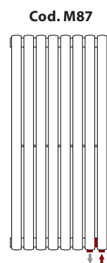
Connection with welded couplings, 50 mm pitch, on the right side
