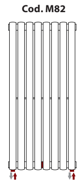
Connection with couplings welded at the ends with diaphragm
